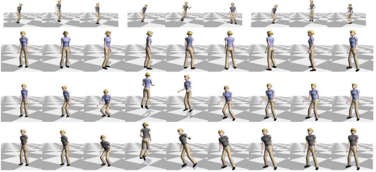
Figure 4: Synthesizing a vertical jump with a 360^\circ turn. (Top row) Motion capture data used to compute the low-dimensional space for the optimization: a forward jump, a forward jump with a 90^\circ turn, and a vertical jump with a 180^\circ turn. (Second row) Initial guess. Constraints were set on the first and the last pose of the motion and on the position of the feet during the stance phases. The duration of each stance phase and the desired height of the jump were also specified. (Third row) Synthesized motion. (Last row) Motion capture data of a similar motion for comparison.
